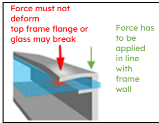
Figure 1a: Clamp Force Locations
