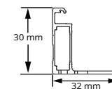
SIDE FRAME PROFILE
