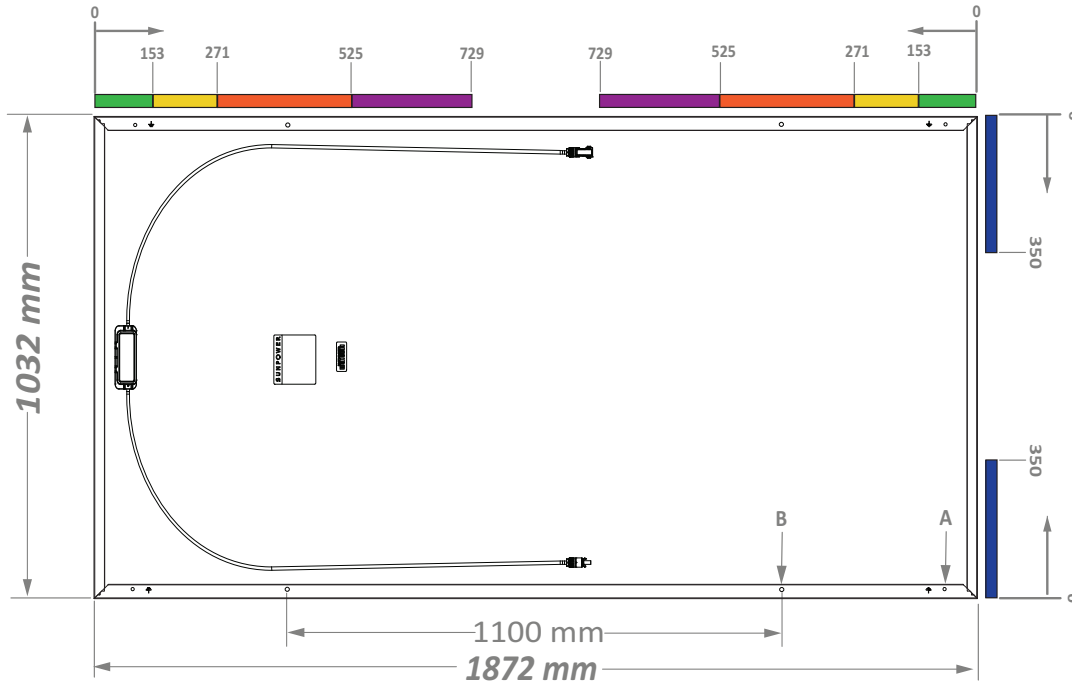
A - Ground Holes (4X Ø4.2mm) B - Mounting Holes (4X Ø6.8mm)
