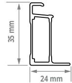
END FRAME PROFILE
