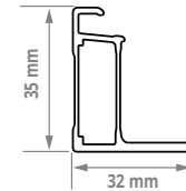
SIDE FRAME PROFILE
